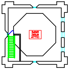
BELFRY PLAN LEVEL 5
