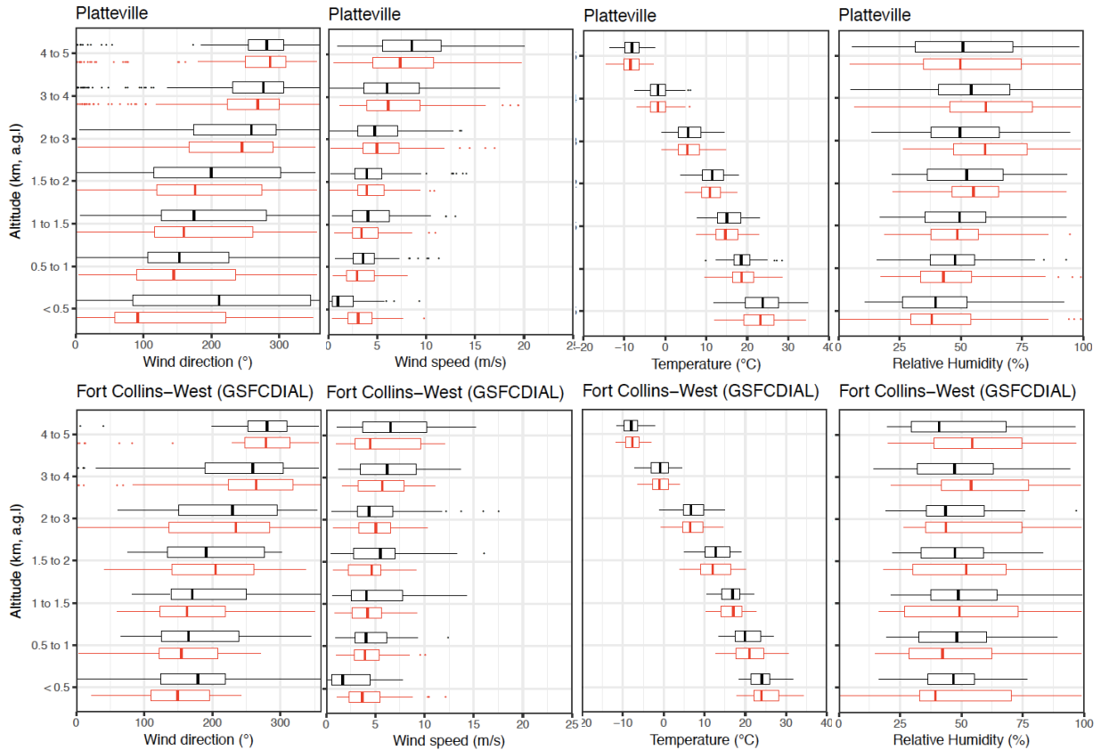
Figure 1: Vertical average profiles for measured (black) and modeled (red) wind direction and wind speed, temperature and relative humidity for ozone sonde launches in Platteville (top) and Fort Collins West (bottom).
